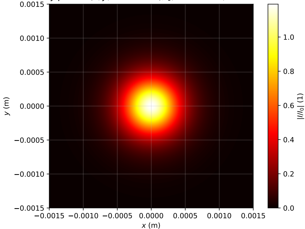
Intensity profile I(x, y, z = 1.513m)/I_0 , P_{in}=0.7P_{cr} , artificial time
